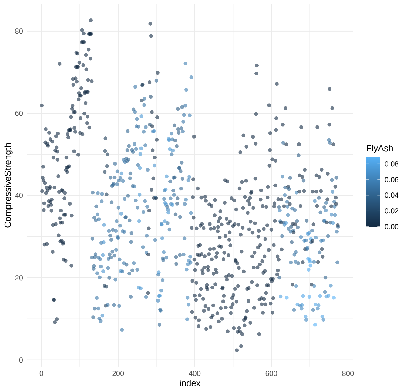
CompressiveStrength vs Index colored by FlyAsh
