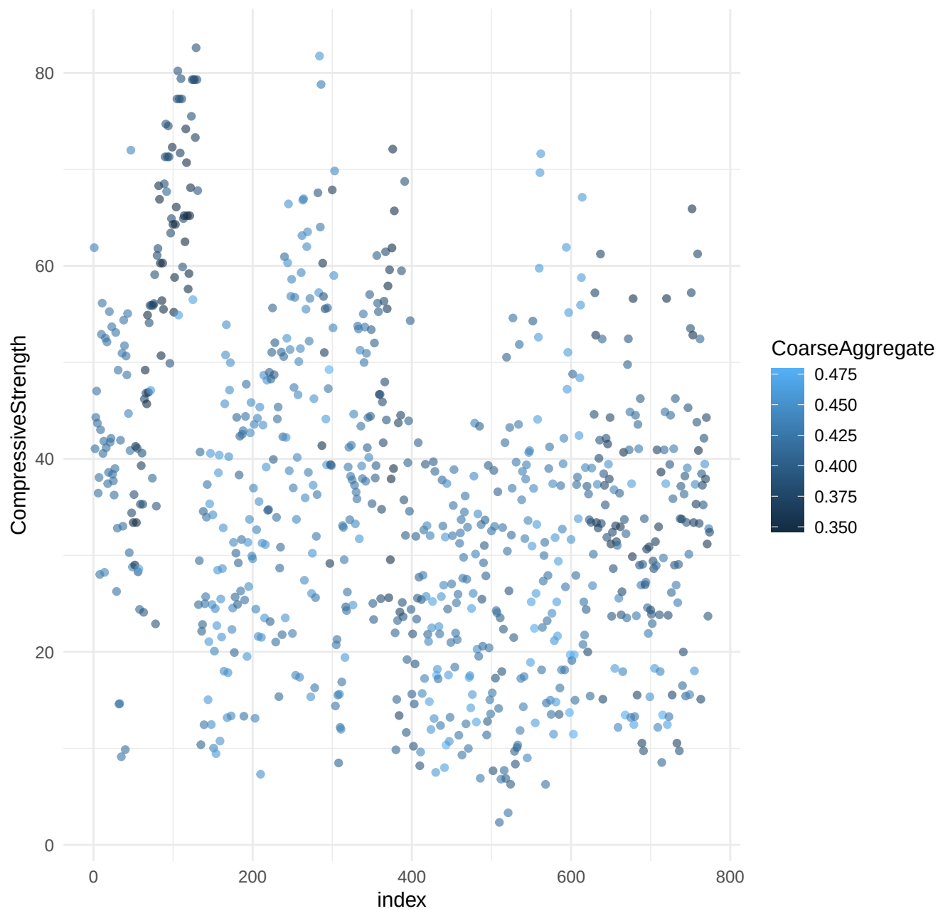
CompressiveStrength vs Index colored by CoarseAggregate
