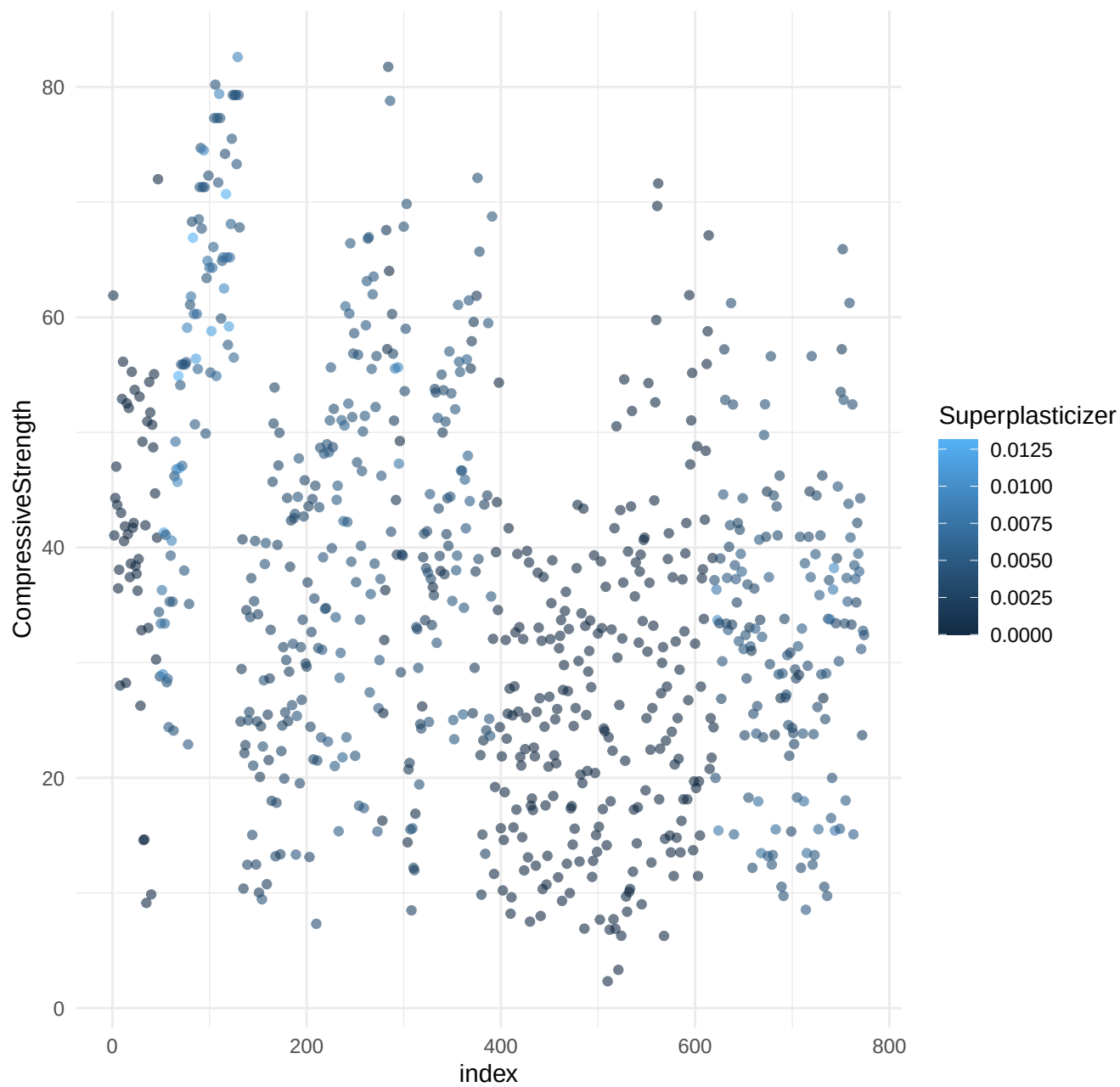
CompressiveStrength vs Index colored by Superplasticizer
