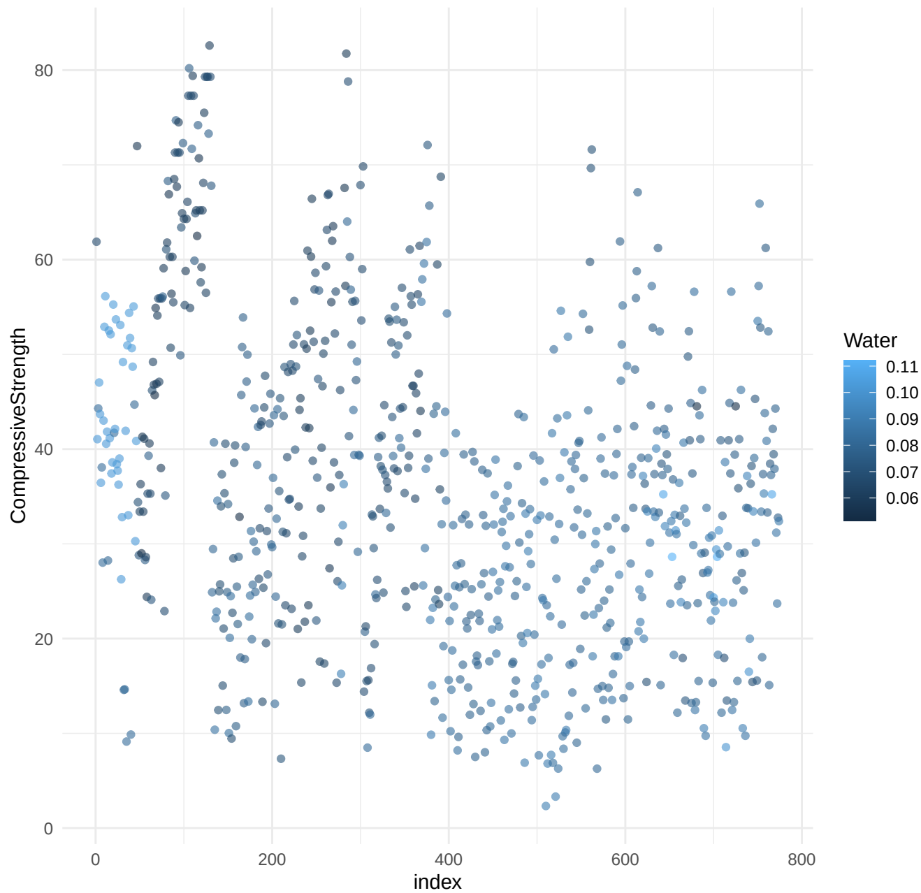
CompressiveStrength vs Index colored by Water
