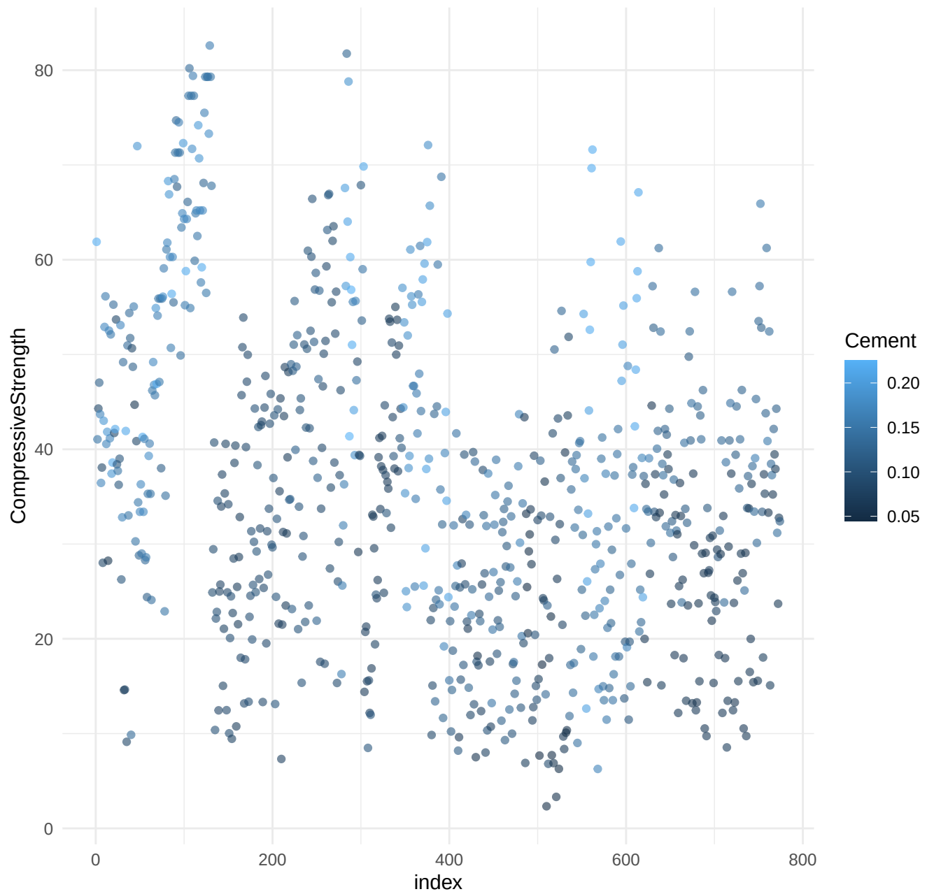
CompressiveStrength vs Index colored by Cement
