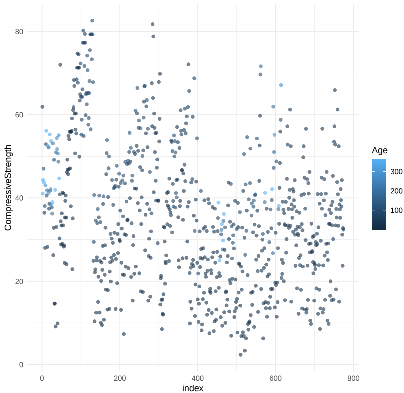
CompressiveStrength vs Index colored by Age
