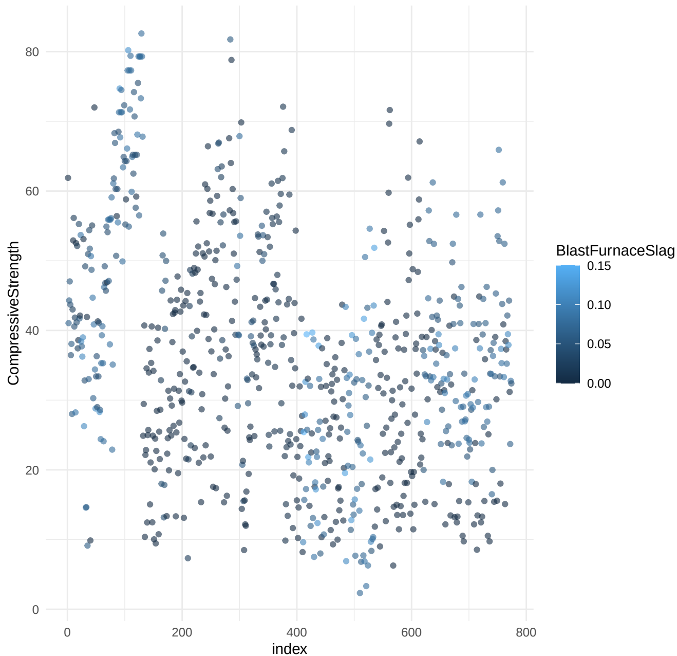
CompressiveStrength vs Index colored by BlastFurnaceSlag
