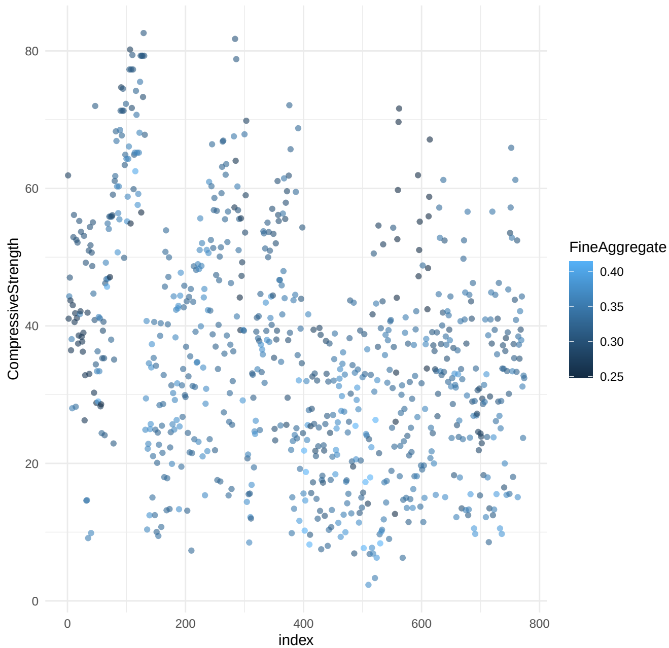
CompressiveStrength vs Index colored by FineAggregate
